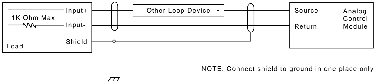
Figure 31: Analog Control Point Wiring
