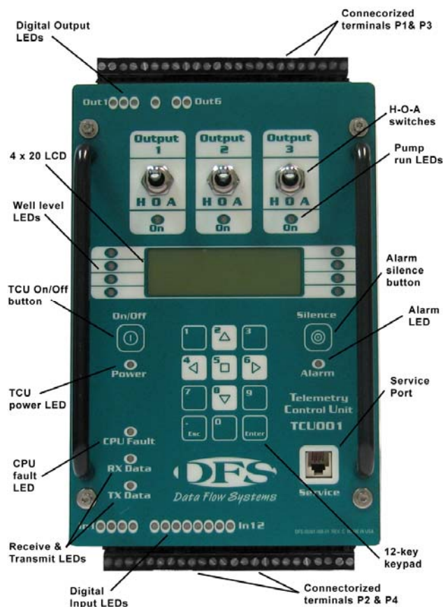
Figure 20: Telemetry Control Unit (TCU)
