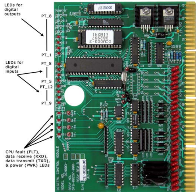
Figure 9: Digital Control Module
