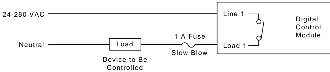
Figure 26: Digital Control Module Wiring
