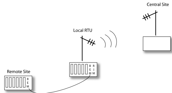
Figure 7: Typical BEM Installation
