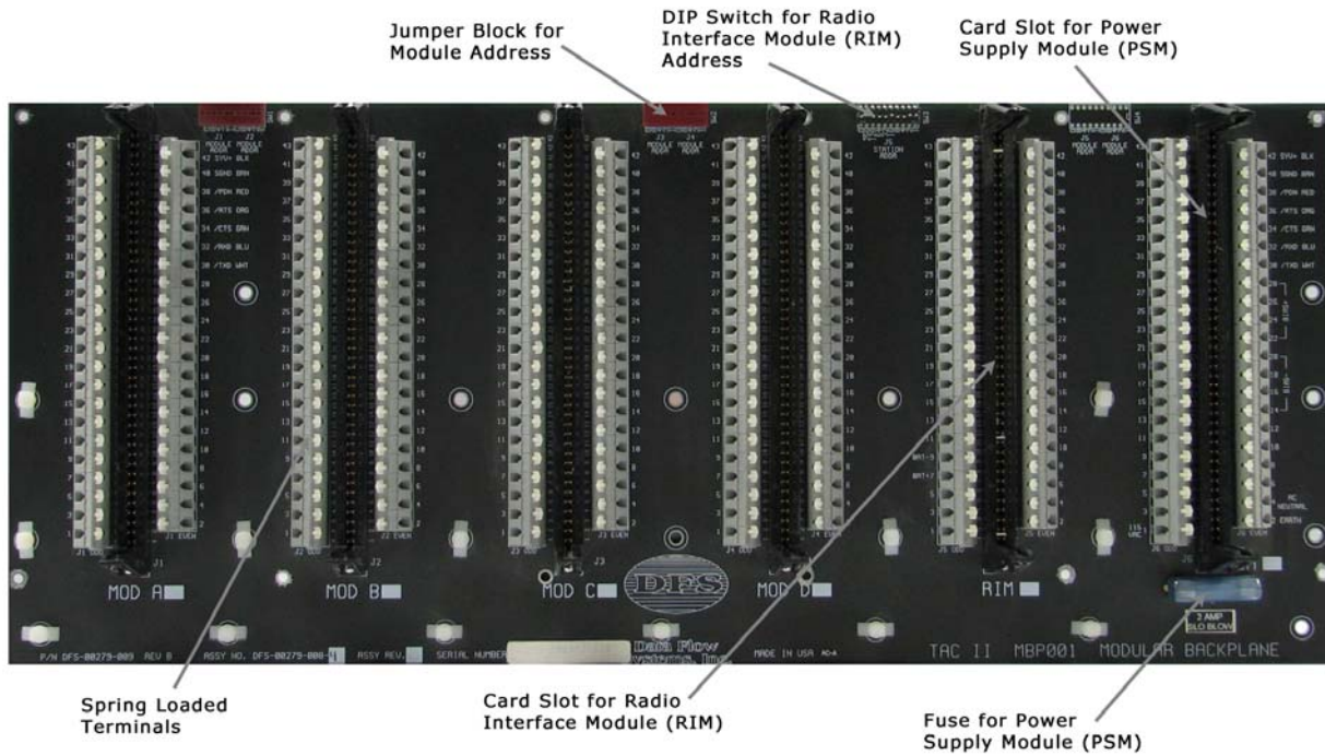
Figure 2: Modular Backplane
