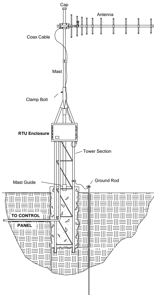
Figure 23: Typical Antenna Tower Installation
