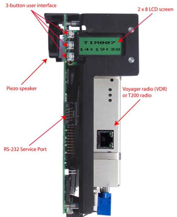
Figure 21: Telemetry Interface Module
