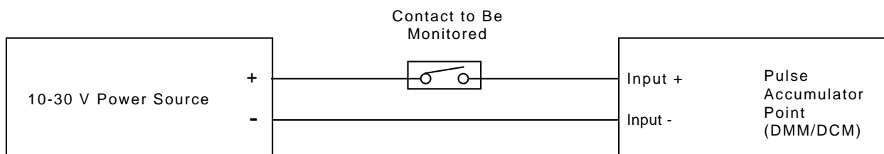
Figure 27: Digital Module Wiring (DCM/DMM) for 10-30V Pulse Accumulator Point
