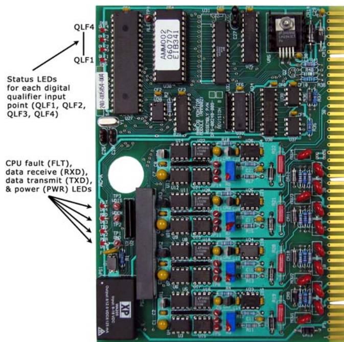
Figure 6: Analog Monitor Module
