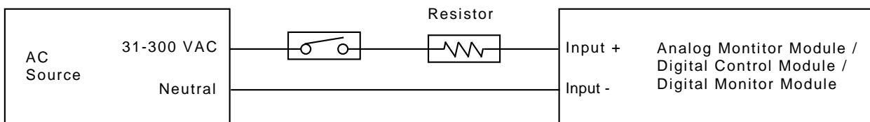
Figure 25: Digital Monitor Module Wiring for High Voltage Monitoring
