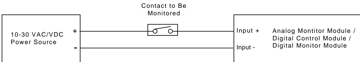
Figure 24: Digital Monitor Module Wiring for Low Voltage Monitoring
