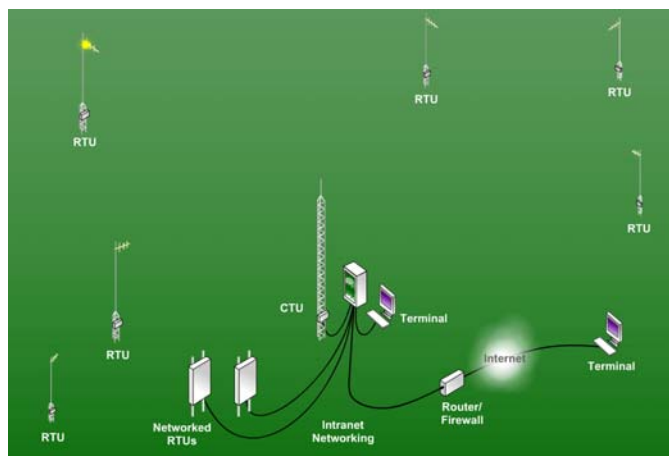
Figure 1: Typical TAC II SCADA System
