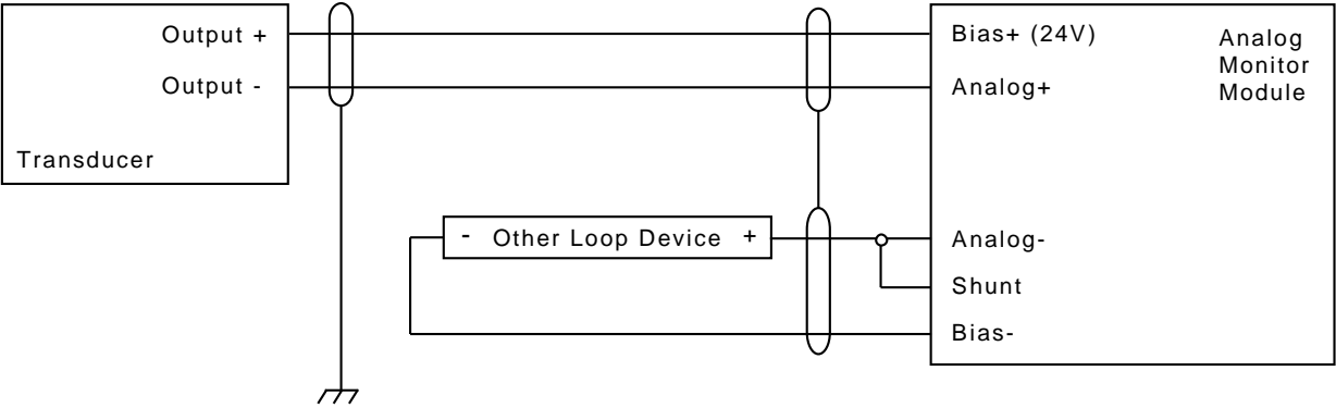
Figure 29: Analog Monitor Point Wiring (0-20 mA Current with AMM-supplied Power)
