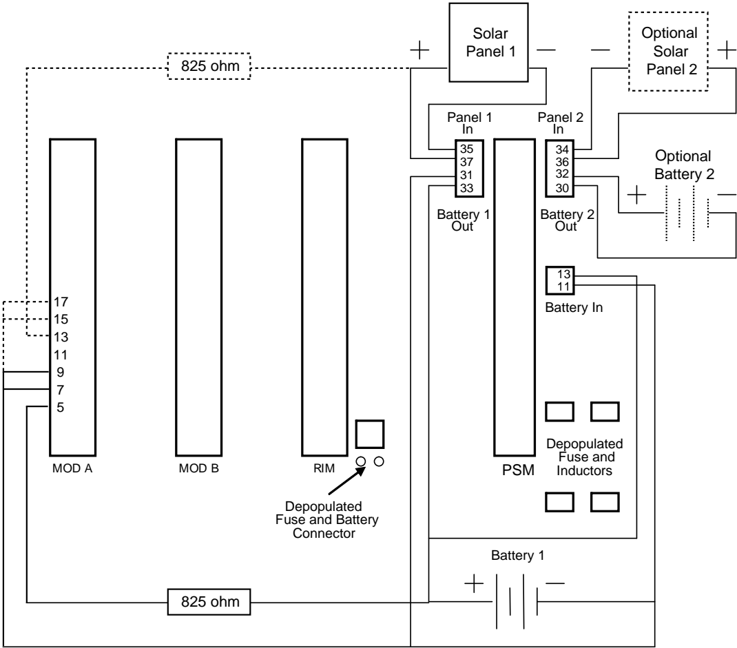
Figure 36: Solar Power Module Wiring
