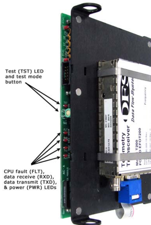
Figure 17: Radio Interface Module (View 2)
