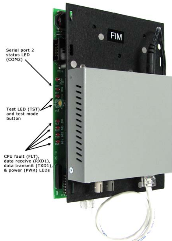
Figure 12: Fiber Interface Module (View 2)
