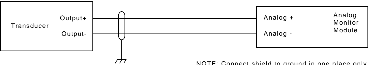
Figure 30: Analog Monitor Point Wiring (0-5 Volt)
