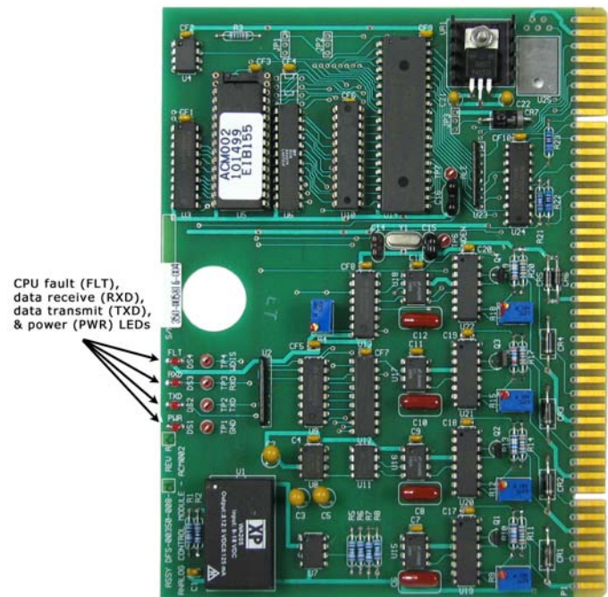
Figure 5: Analog Control Module
