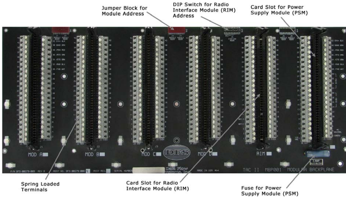
Figure 33: Modular Backplane (MBP001) Used in RTU204
