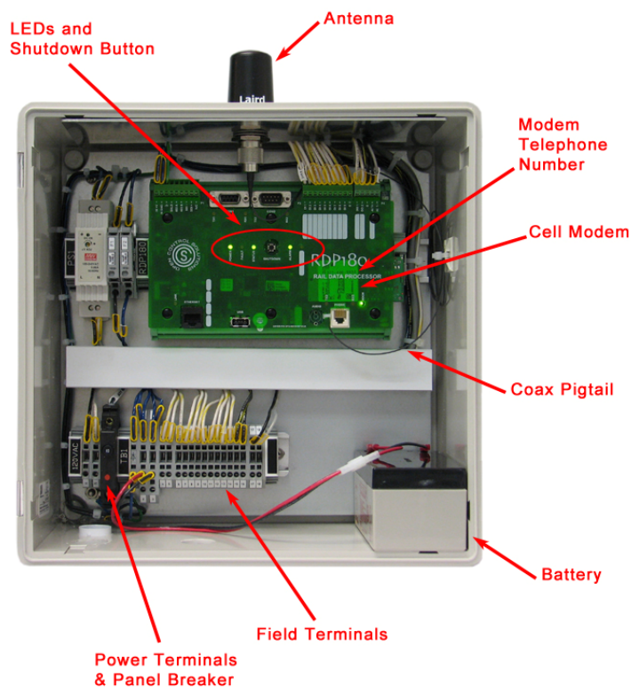
Figure 18: RDP180-C (Cellular RTU)
