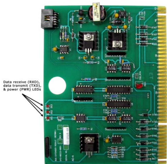
Figure 8: Bus Extender Module
