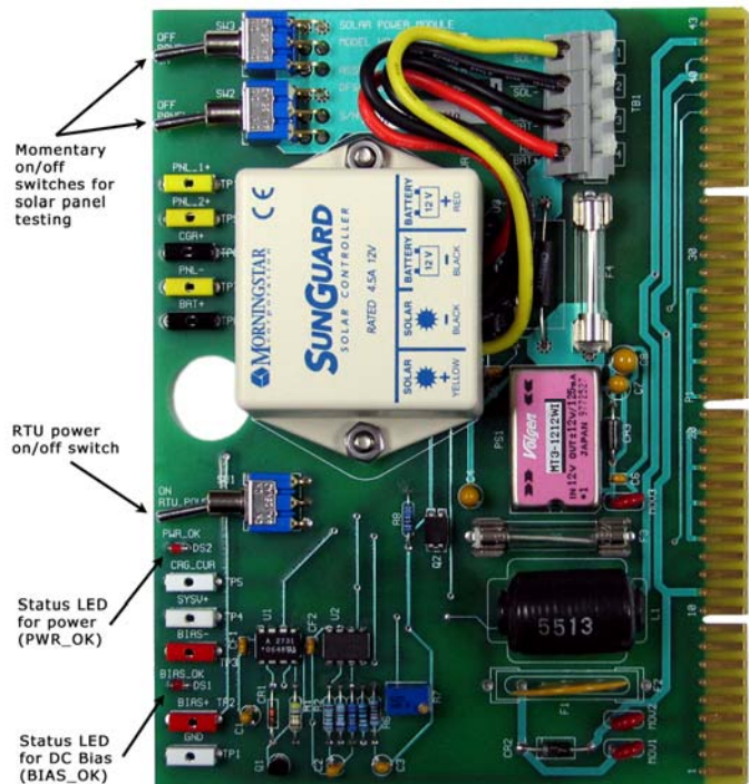
Figure 19: Solar Power Module
